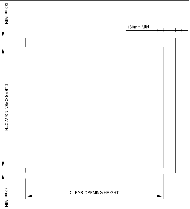
DETAIL SHOWING MINIMUM JAMB & HEAD SURFACE DIMENSIONS
