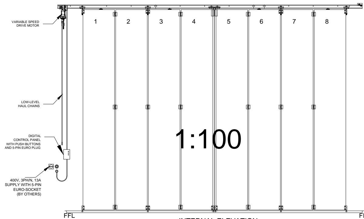
INTERNAL ELEVATION SHOWING STANDARD HARDWARE OPTIONS (AS DRAWN 4+4 LEAVES)
