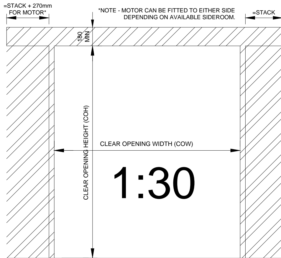
ELEVATION SHOWING INSIDE FACE OF DOOR FRAME
