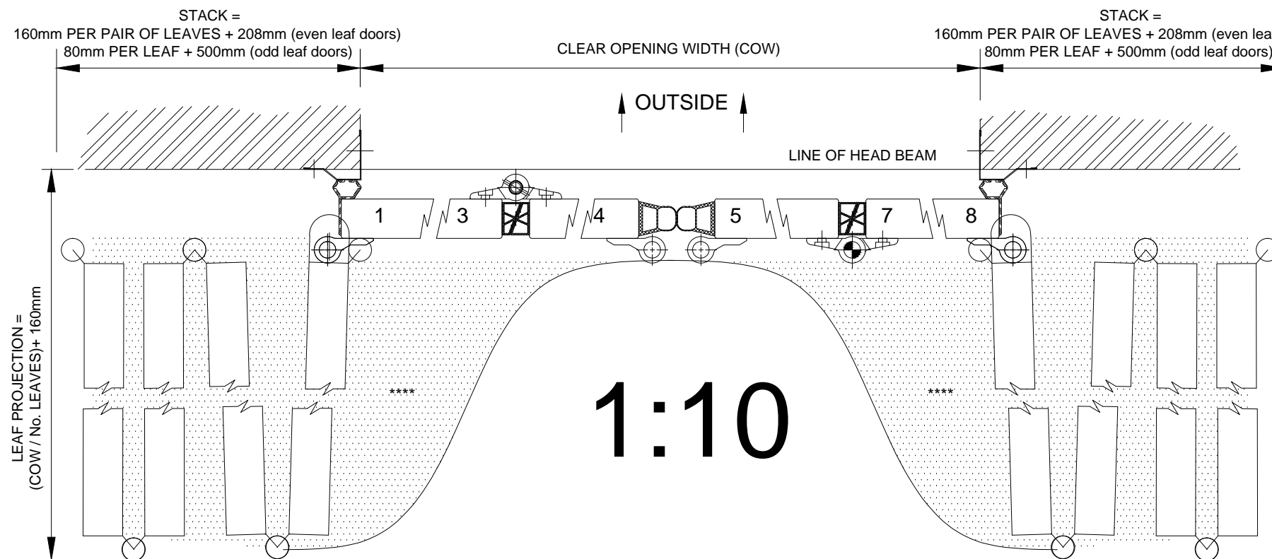
PLAN OF DOOR PANELS IN OPEN AND CLOSED POSITIONS
