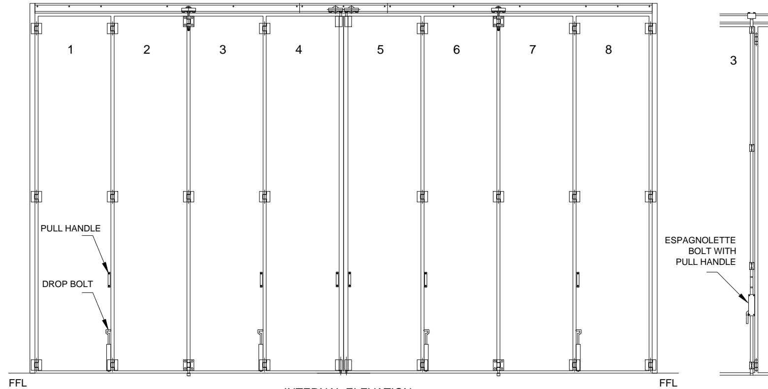
INTERNAL ELEVATION SHOWING LOCKING OPTION
