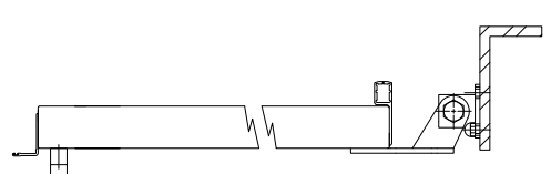
DETAIL SHOWING PULL HANDLE FITTED TO ACTIVE LEAF
