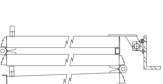
DETAIL SHOWING PULL HANDLE FITTED TO ACTIVE LEAF
